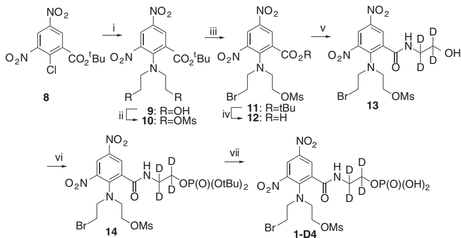
Scheme 3 Synthesis of 2H4 PR-104.
